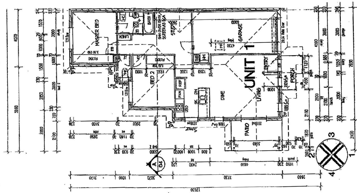
FLOOR PLAN SCALE 1:100 PRECUTTER AND CARPET AND LINEN DOOR OPENING TRIM STUD'S REG'D.
